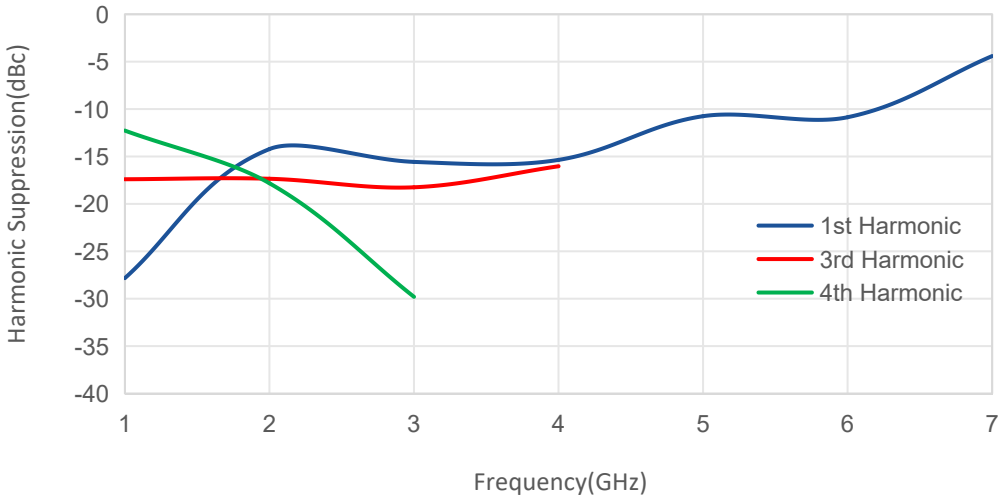
Harmonic Suppression vs Frequency@Pin=-1dBm
