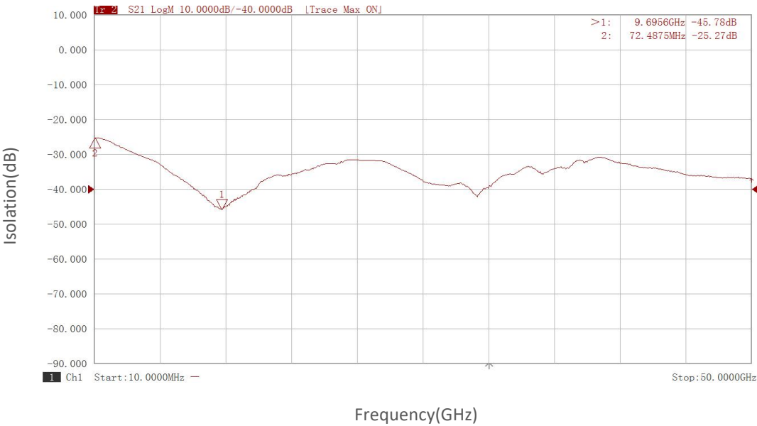
LO to IF Isolation vs Frequency
