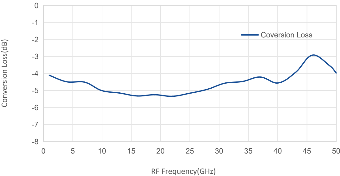
Coverison Loss vs RF Frequency
