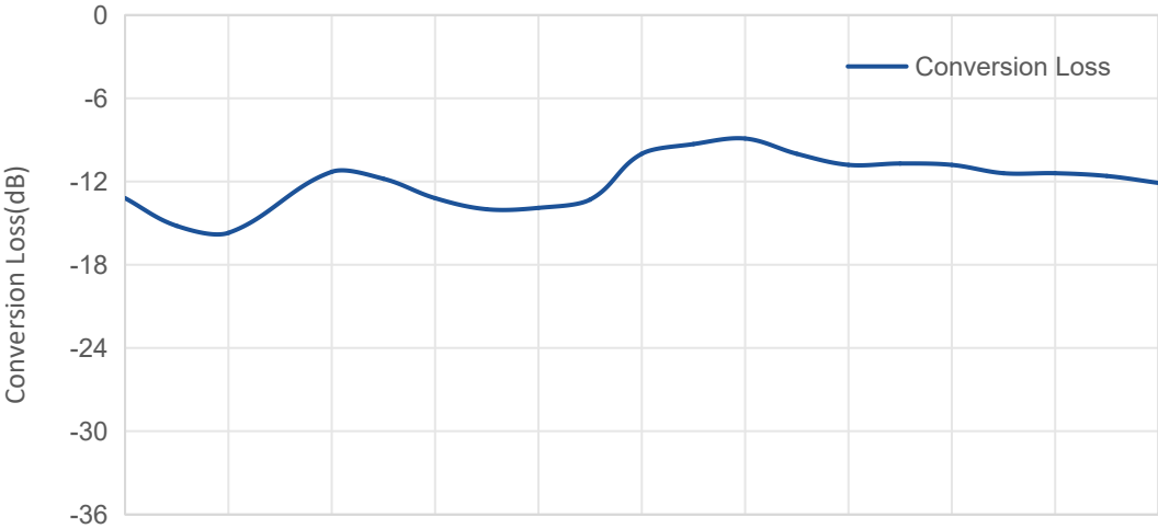
Conversion Loss vs RF Frequency
