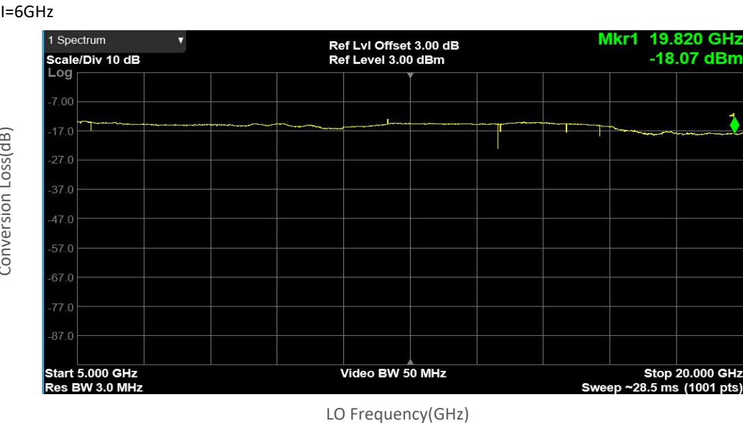
Conversion Loss vs LO Frequency
