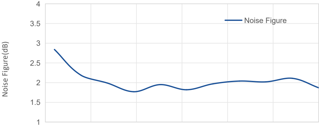
Noise Figure vs Frequency
