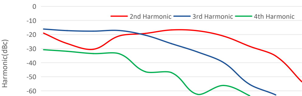
Harmonics vs Frequency
