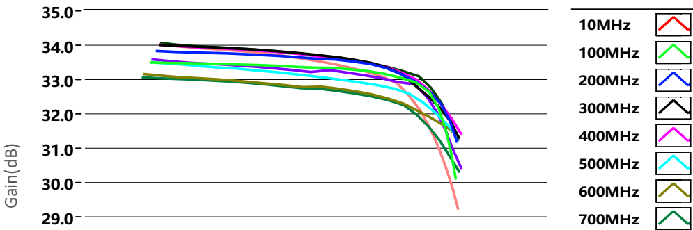
Gain vs Output Power
