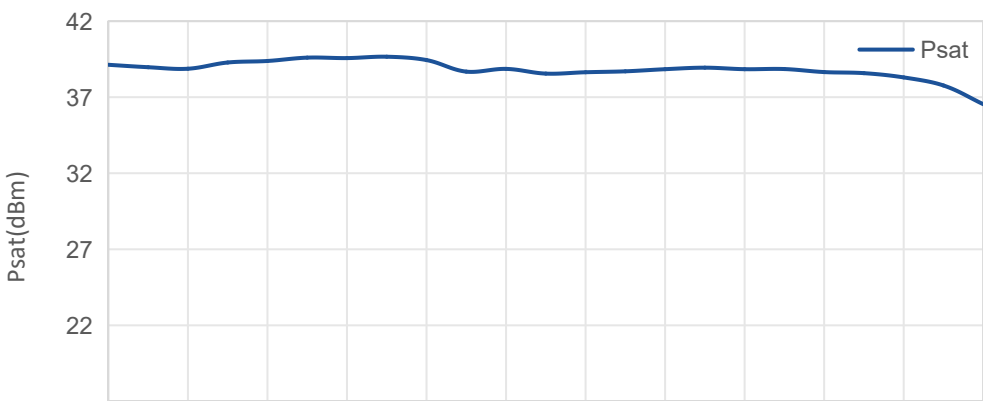
Psat vs Frequency
