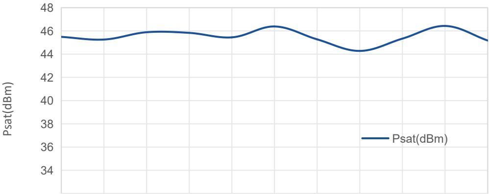
Psat vs Frequency
