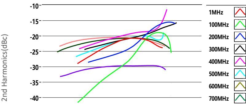
2nd Harmonics vs Output Power
