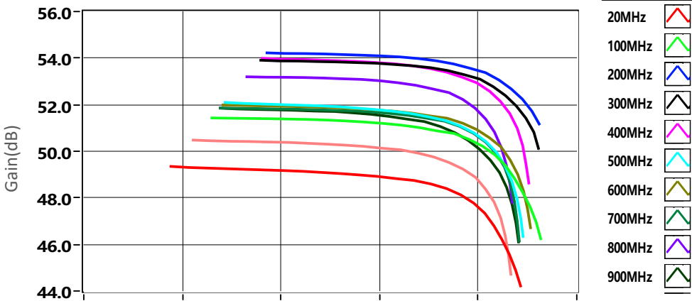
Gain vs Output Power
