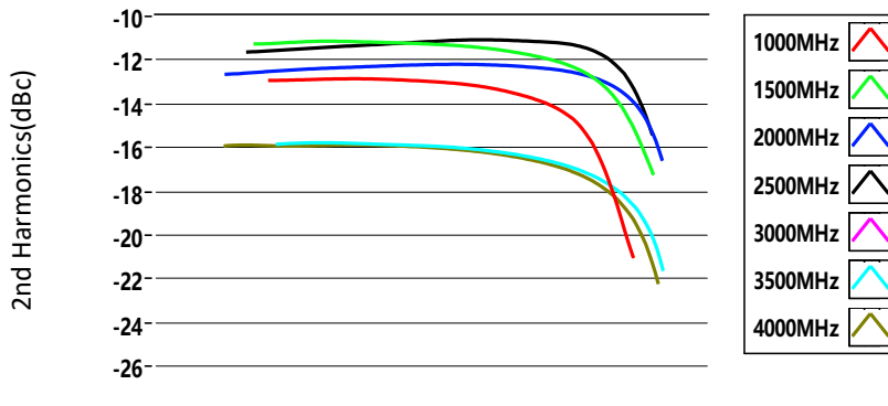
2nd Harmonics VS Output Power
