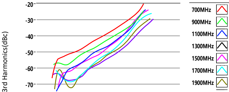
3rd Harmonics VS Output Power
