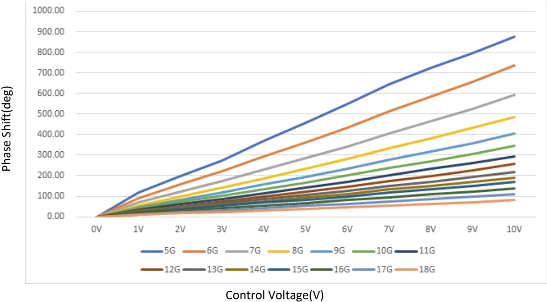
Phase Shift vs Control Voltage
