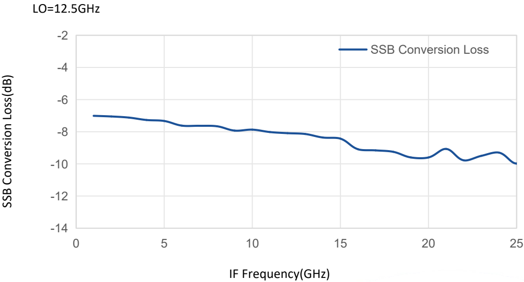
SSB Covernion Loss vs IF Frequency
