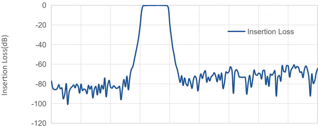
Insertion Loss vs Frequency
