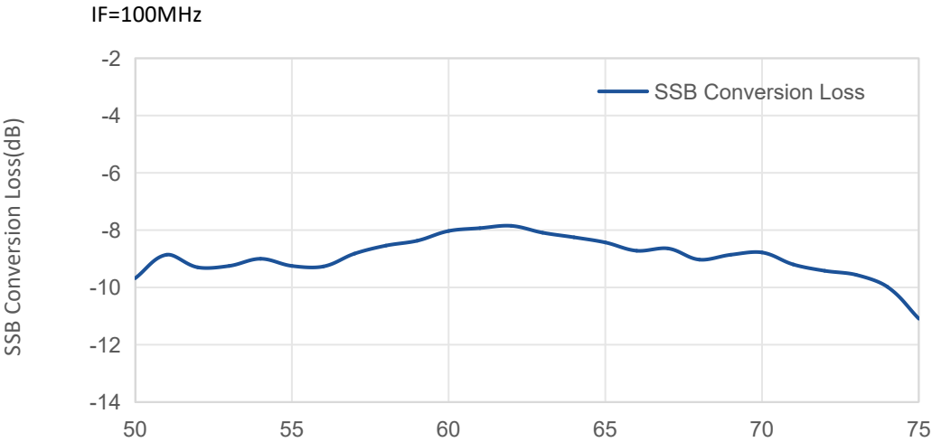
SSB Covoersion Loss vs RF Frequency
