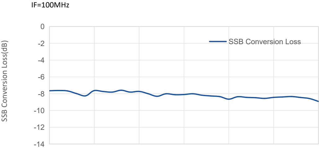
SSB Coversion Loss vs RF Frequency
