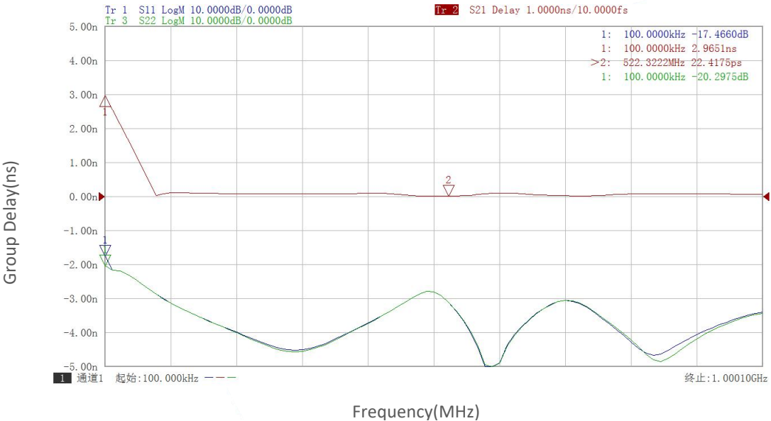
Group Delay vs Frequency
