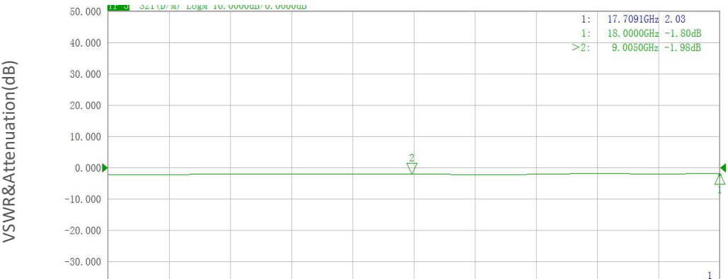
VSWR&Attenuation vs Frequency
