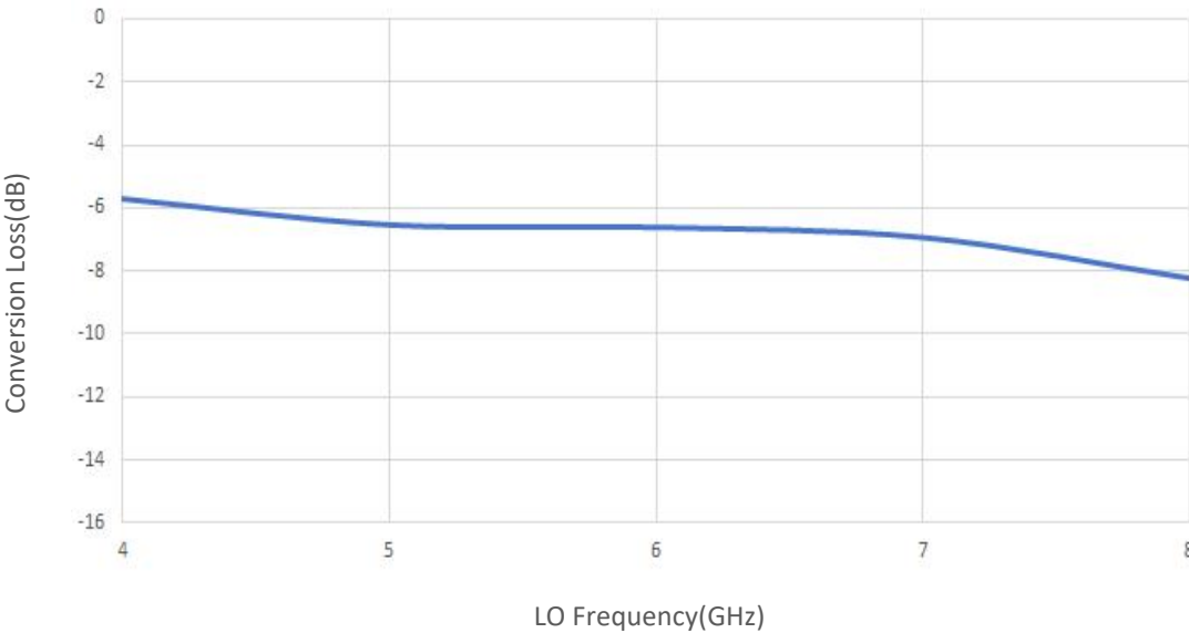
Coverison Loss vs LO Frequency
