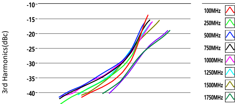
3rd Harmonics VS Output Power
