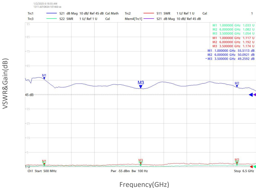
VSWR&Gain vs Frequency
