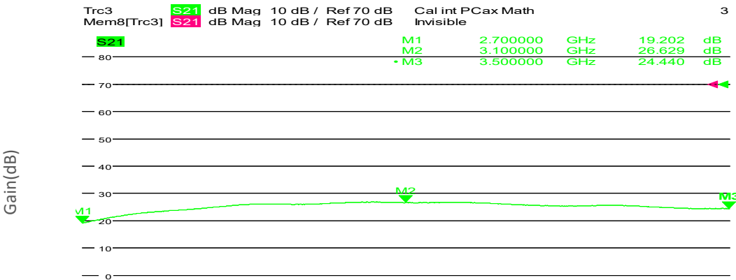
Small Signal Gain vs Frequency
