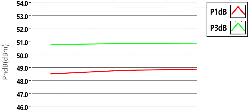
PndB vs Frequency
