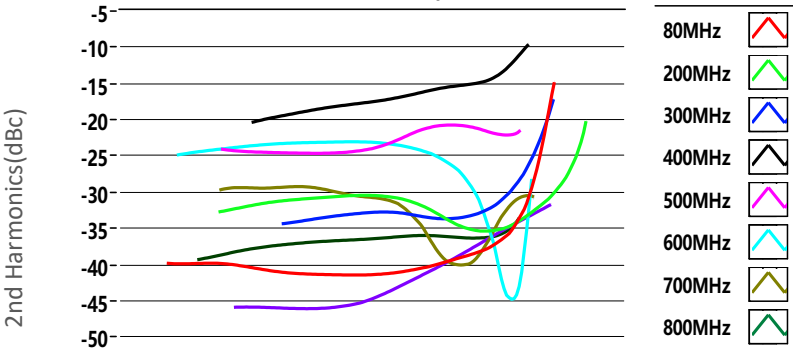
2nd Harmonics vs Output Power
