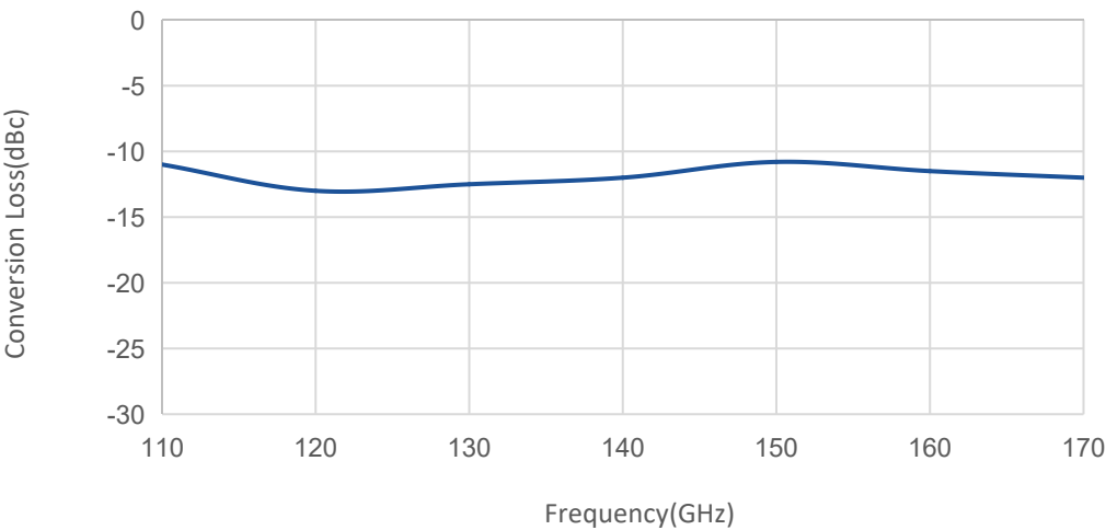
Conversion Loss vs Frequency
