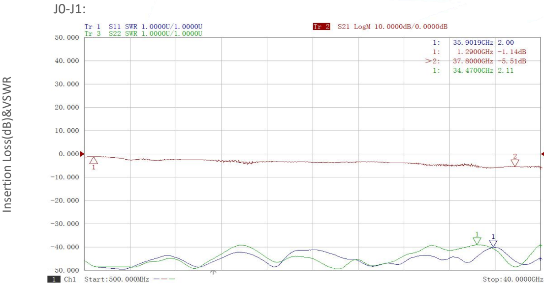
Insertion Loss & VSWR vs Frequency
