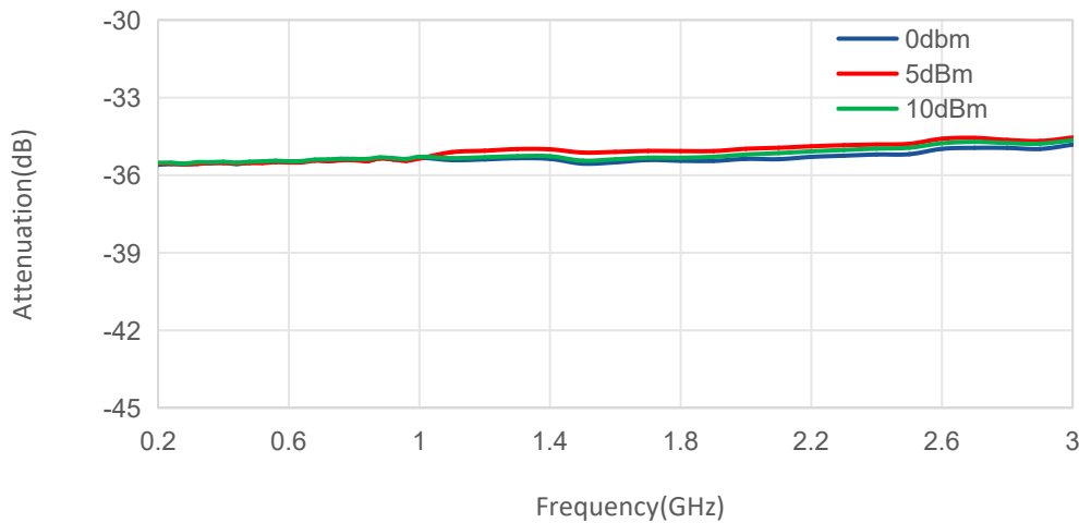
Attenuation@Pin V_T=1V
