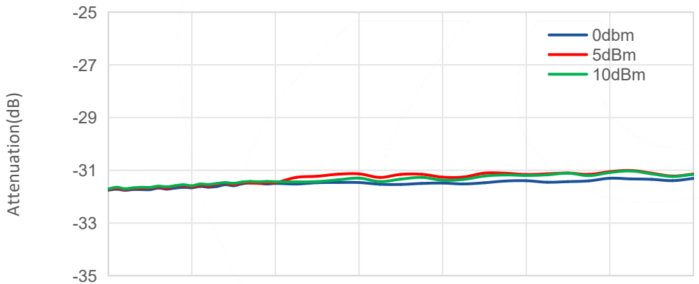
Attenuation@Pin V_T=1.5V
