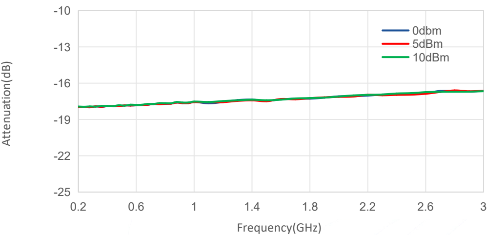
Attenuation@Pin V_T=3V
