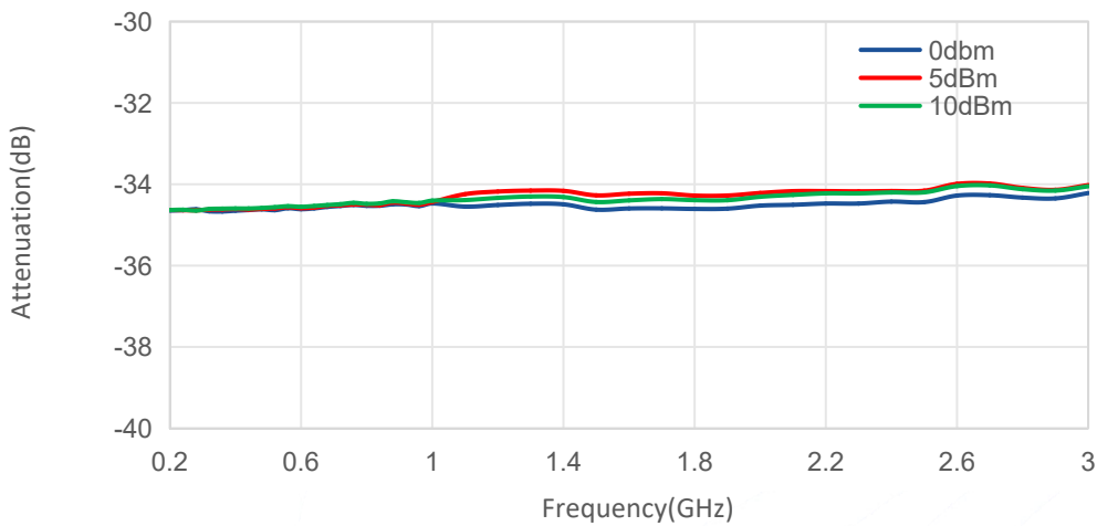
Attenuation@Pin V_T=1.5V
