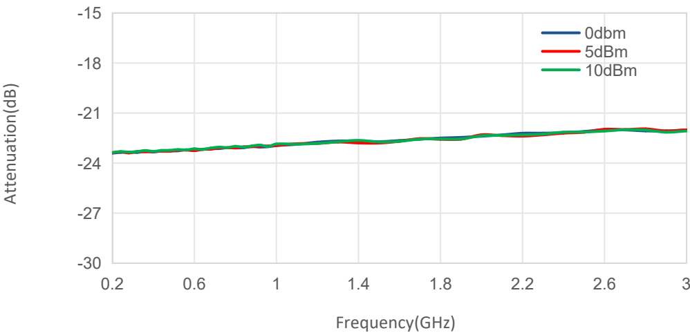
Attenuation@Pin V_T=2.5V
