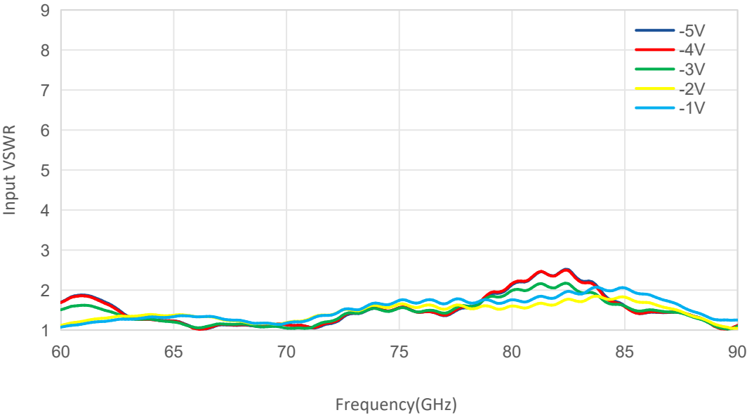
Input VSWR@Voltage
