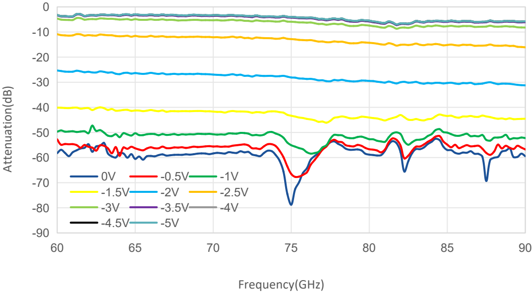
Attenuation@Voltage
