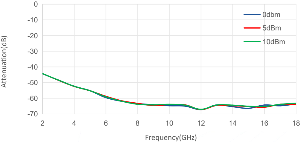
Attenuation@Pin V_T=6V
