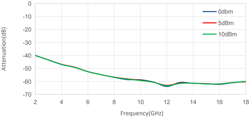
Attenuation@Pin V_T=5V
