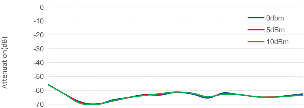
Attenuation@Pin V_T=9V
