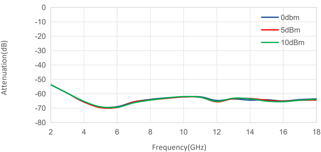
Attenuation@Pin V_T=9V
