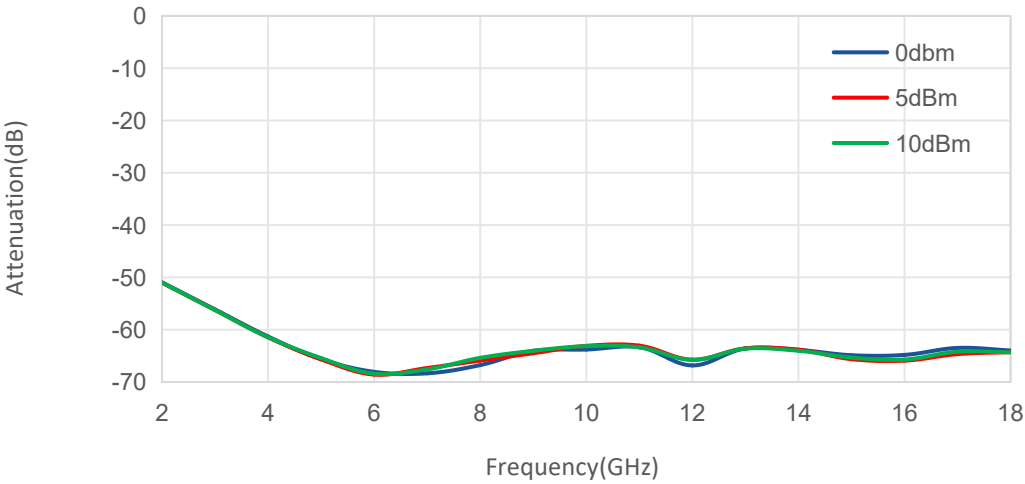
Attenuation@Pin V_T=8V
