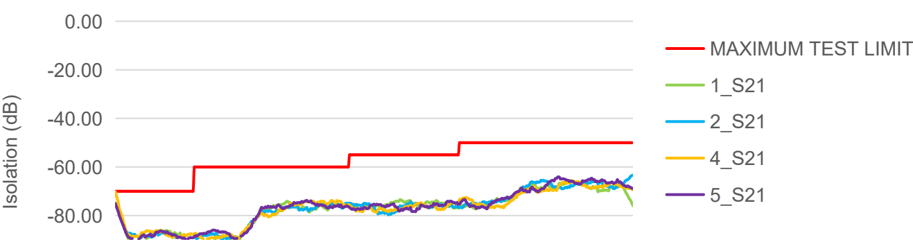
ISOLATION
