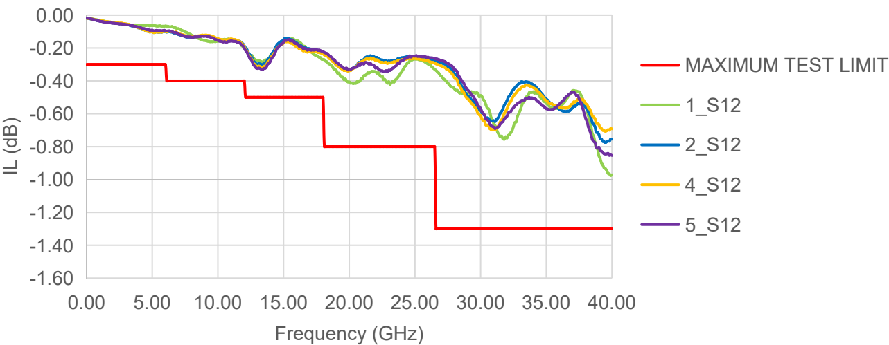
INSERTION LOSS
